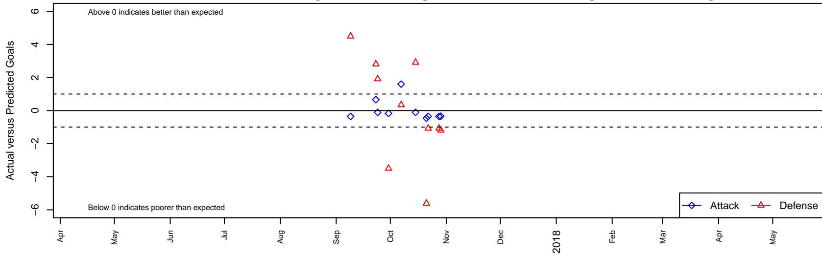
Academia Leon B05 Dots are actual minus expected GF (blue circles) and GA (red triangles). Blue line is smoothed change in attack strength. Red is smoothed change in defense strength.
